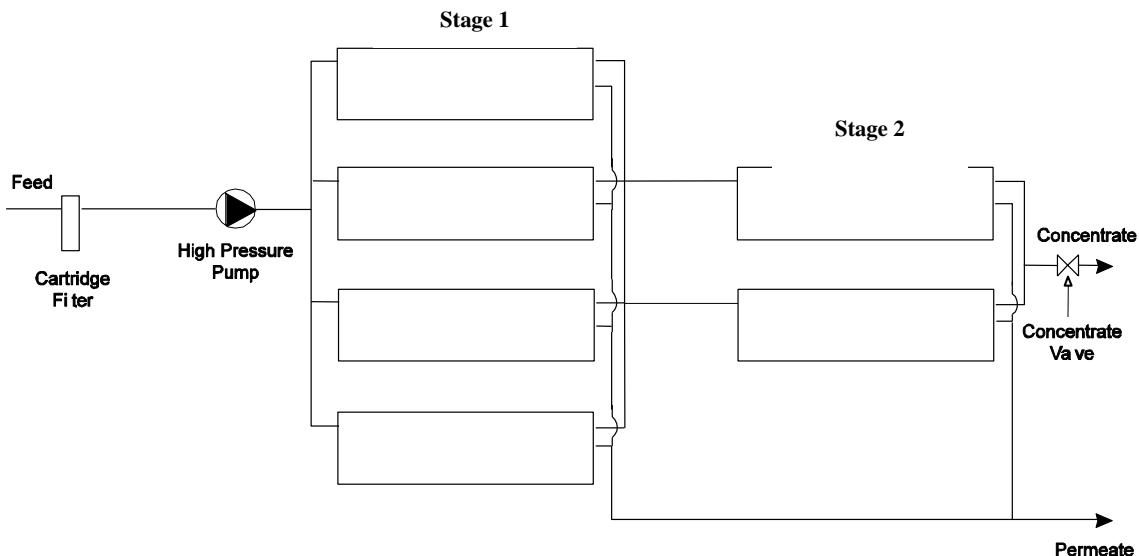
Figure 3.5 Two-stage system
