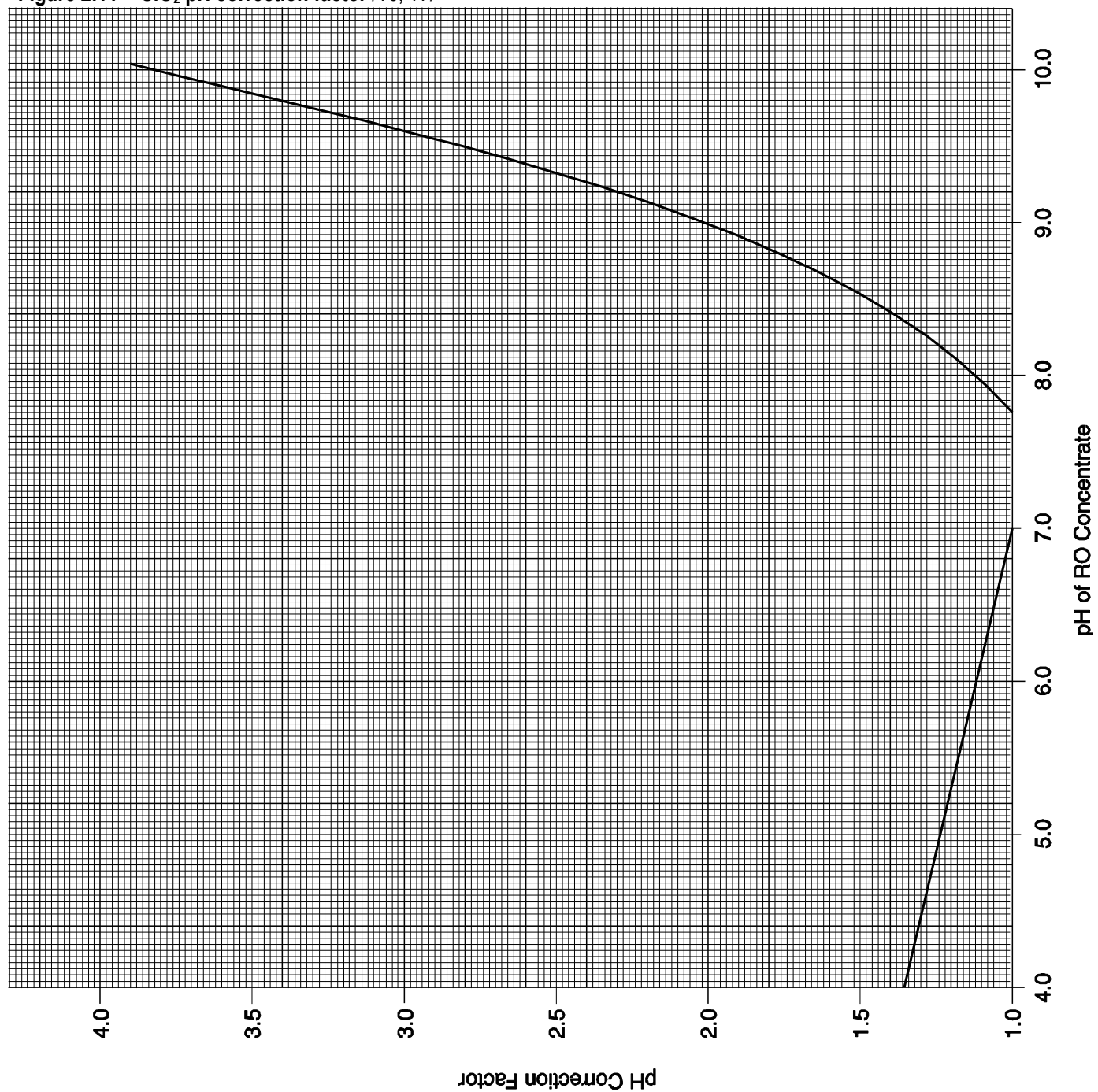
Figure 2.11 \text{SiO}_2 pH correction factor /16, 17/
